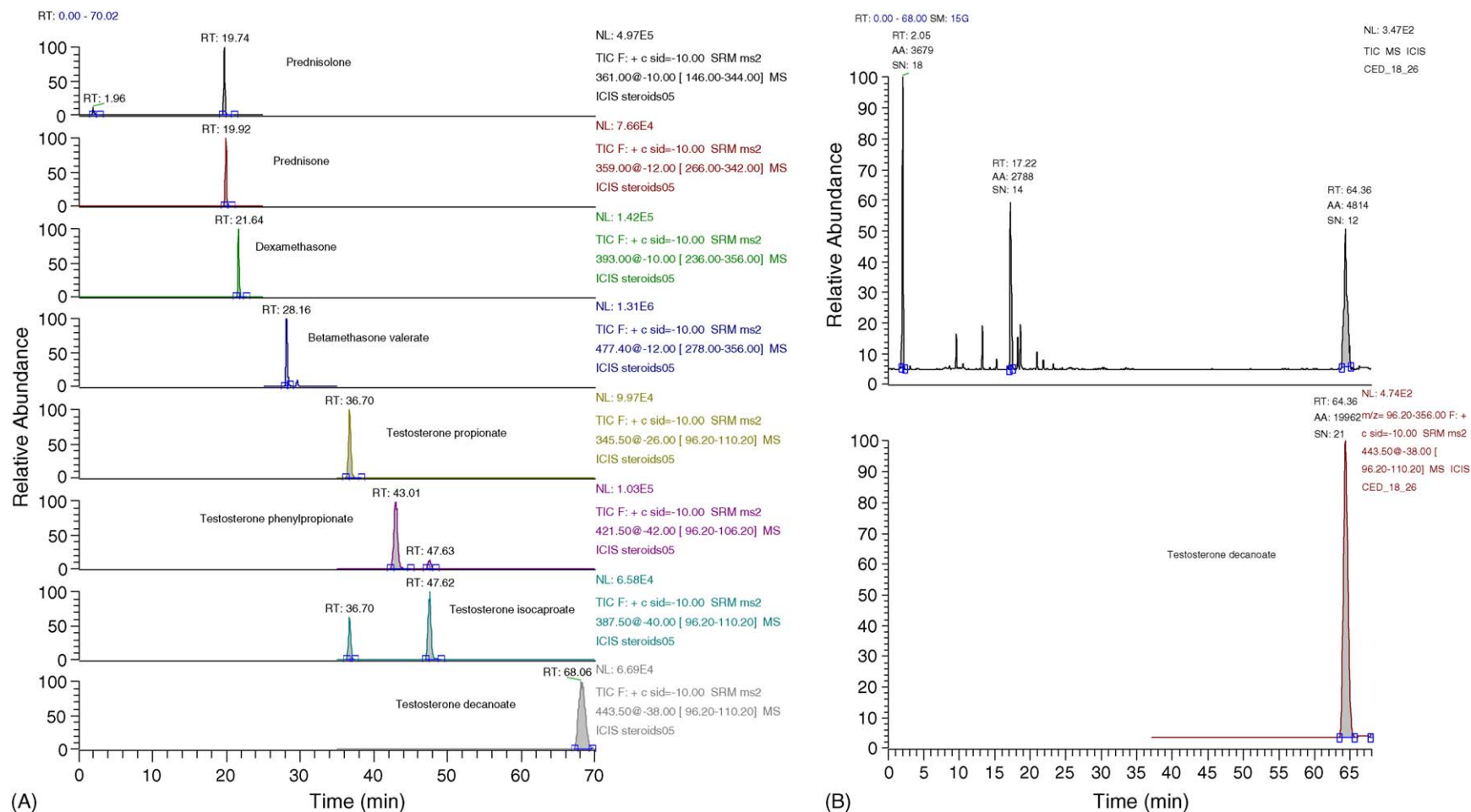
Fig. 3. Mass chromatogram of the mixture of selected steroids (A), mass chromatogram of the extract from Japanese remedy “for female sexuality”, containing testosterone decanoate (B). For each peak, a TIC (total ion chromatogram) of two transitions is shown.
