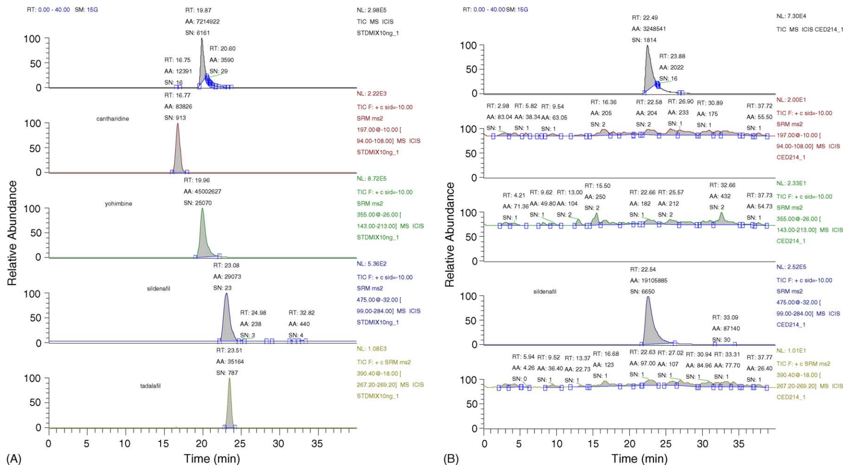
Fig. 4. Mass chromatogram of the mixture of aphrodisiac compounds (A), mass chromatogram of the extract from “herbal” capsules “PhytoAndro”, containing sildenafil (B). For each peak, a TIC (total ion chromatogram) of two transitions is shown.
